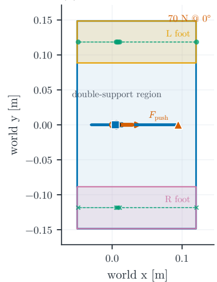
(a) support geometry
