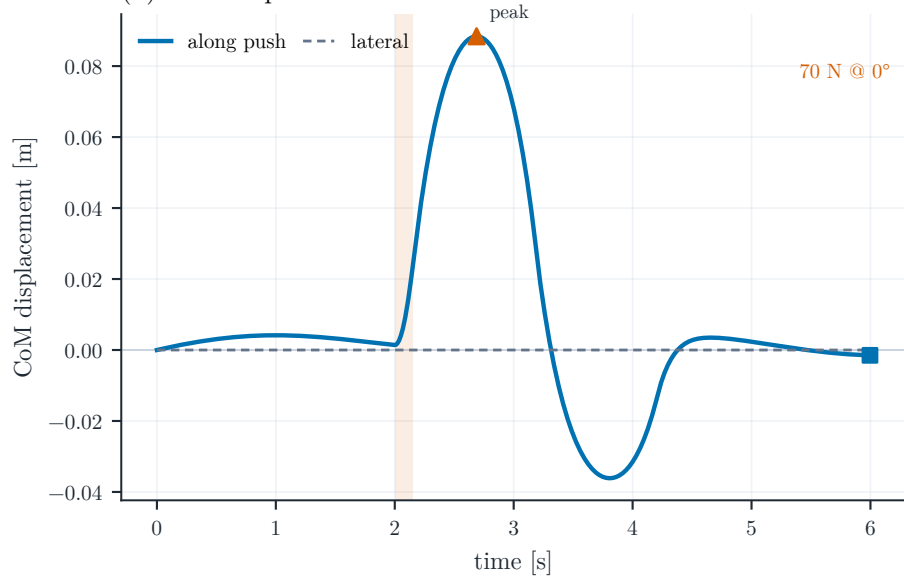
(b) CoM response
