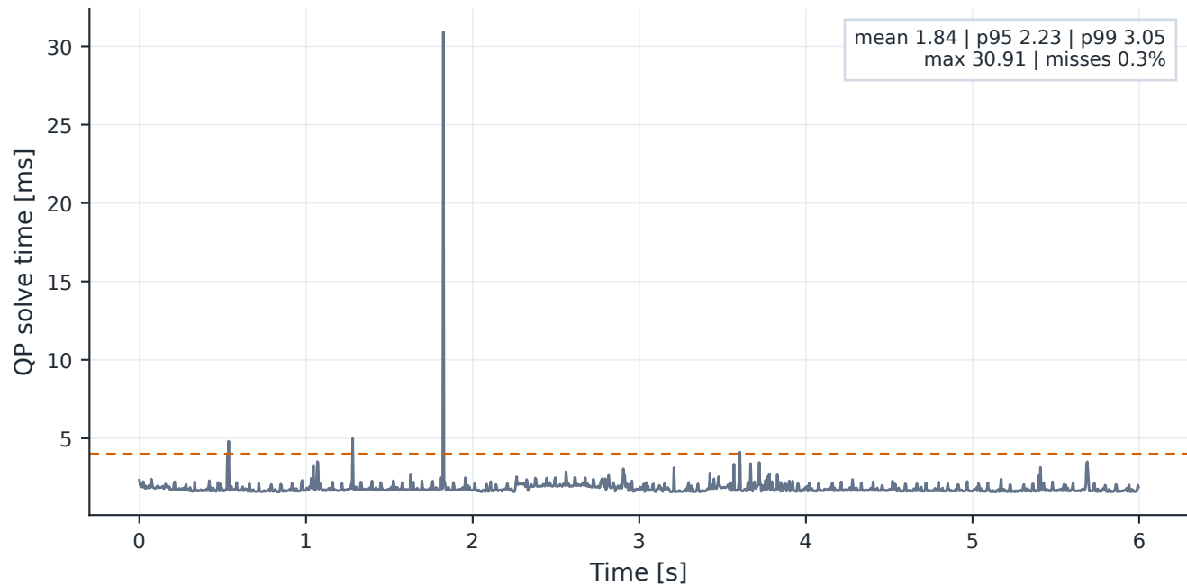
QP timing against the 4 ms control deadline
