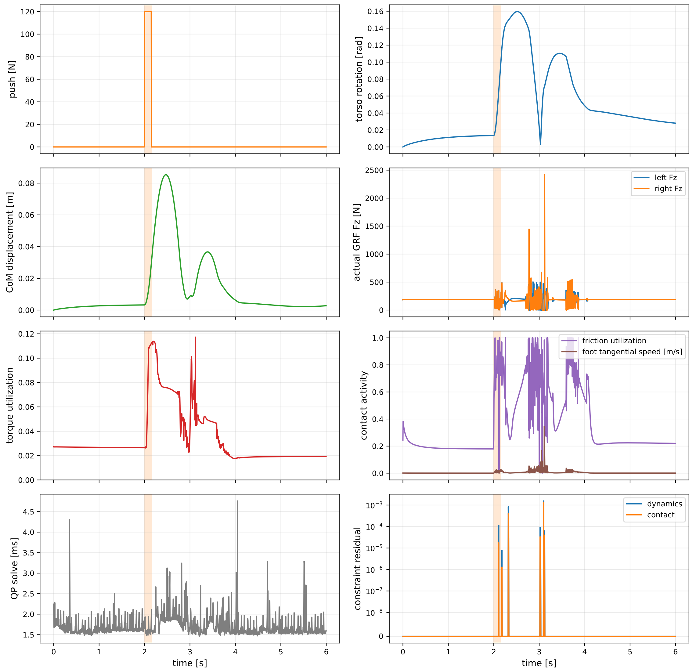
Canonical SE(3) push recovery: measured response and constraints
