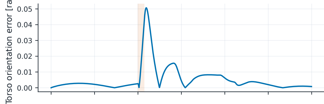
(b) Geometric pose response
