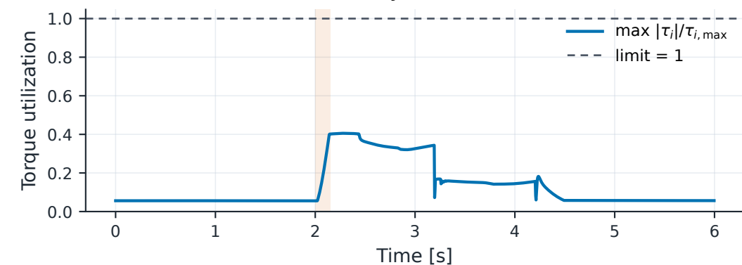
(e) Actuator constraint activity
