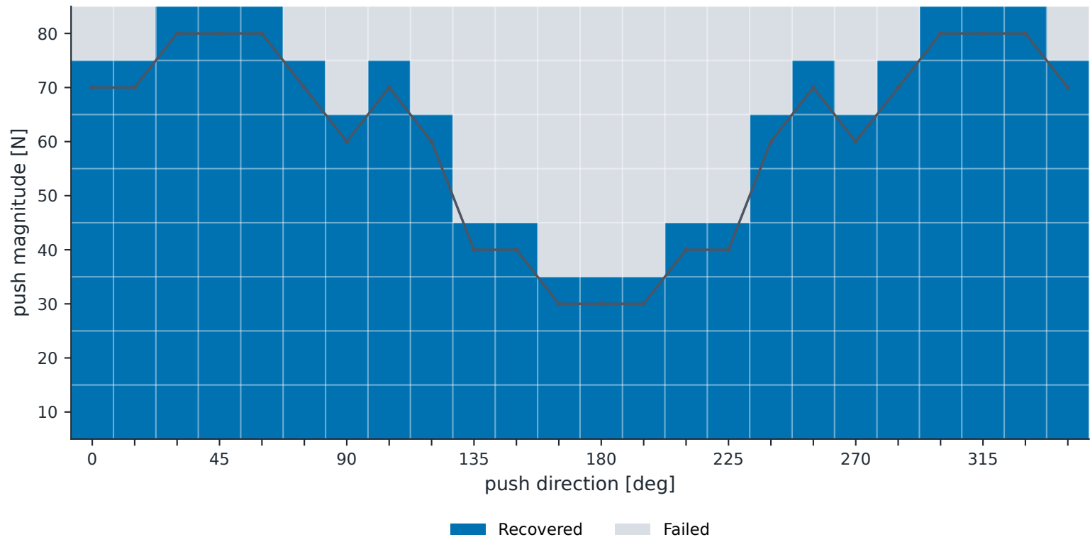
SE(3) WBC recovery basin
