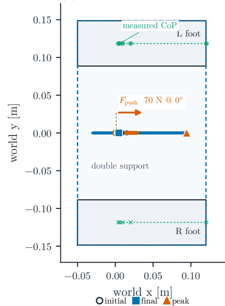
(a) support-plane geometry
