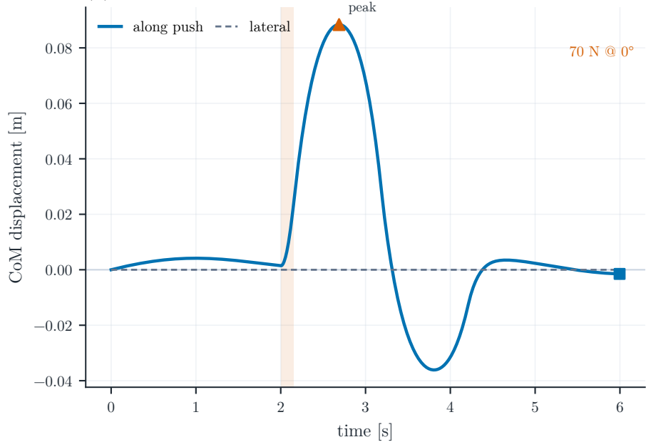
(b) CoM response
