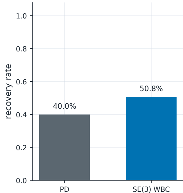
Success over 480 deterministic pushes
