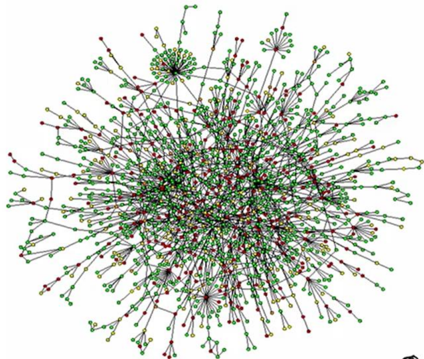
Protein-protein interactions [Jeong et al. 2001]
