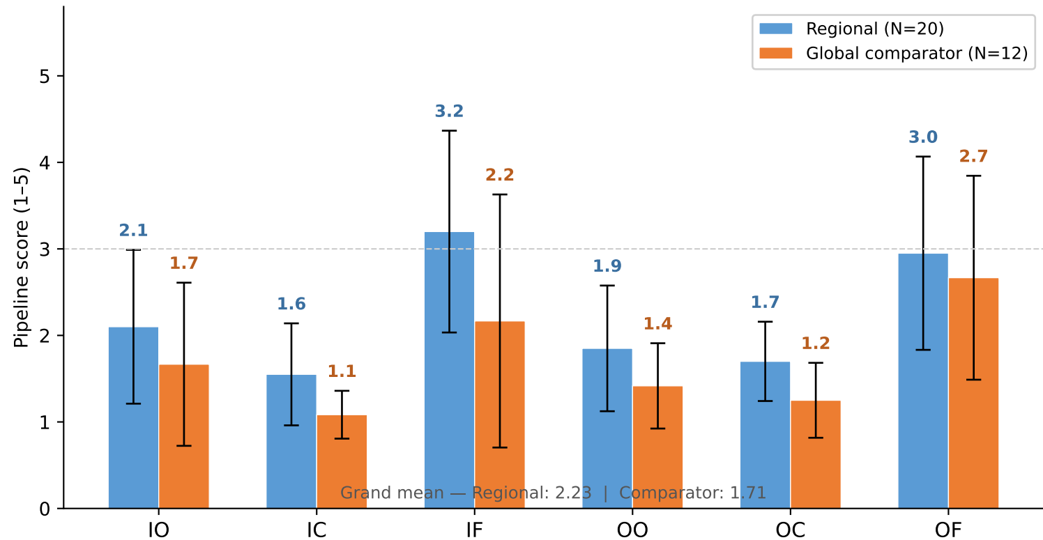
Pipeline Validity Scores: Regional vs. Global Comparator Benchmarks
