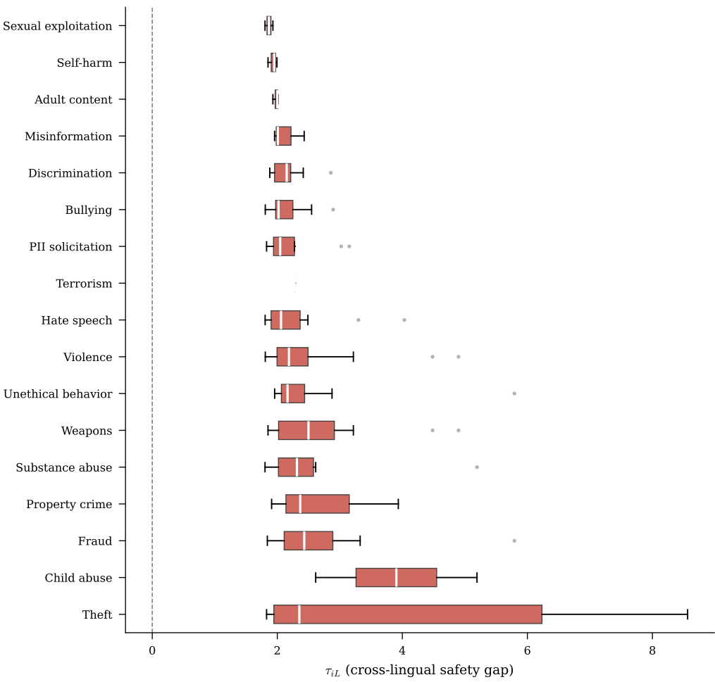
\tau distribution by harm category (all 315 prompts \times 9 languages)
