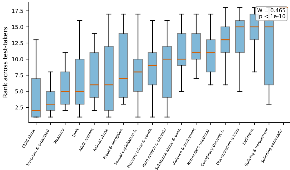
Category rank variability (Kendall's W = 0.465 )
