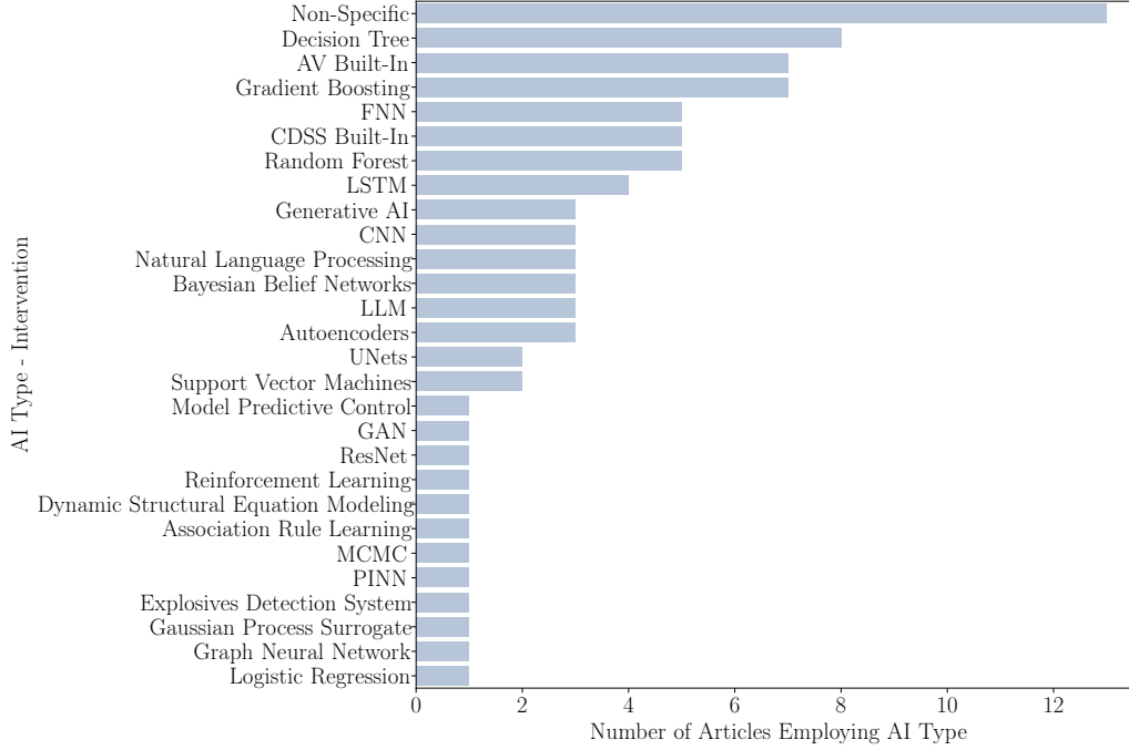
Figure 6: Number of articles in the final subset that considered each type of AI method. Non-specific means the article did not provide details about the model type.
