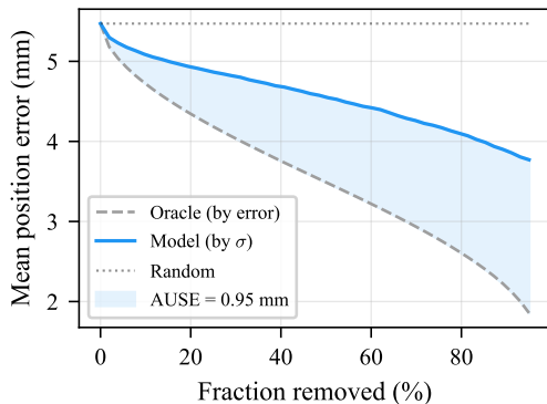
(c) Sparsification curve
