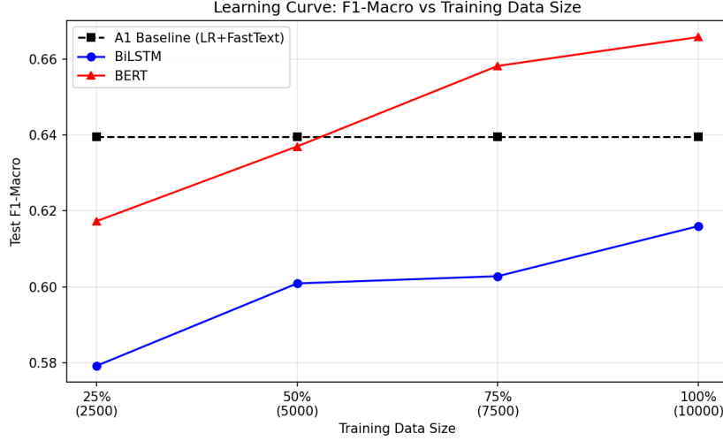
Figure 2: Learning curves for different data percentages. BERT shows much better data efficiency than LSTM.
