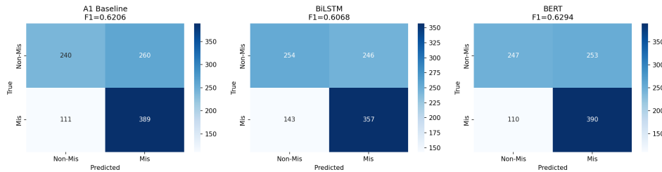
Figure 3: Confusion matrices for BiLSTM and BERT on the test set.
