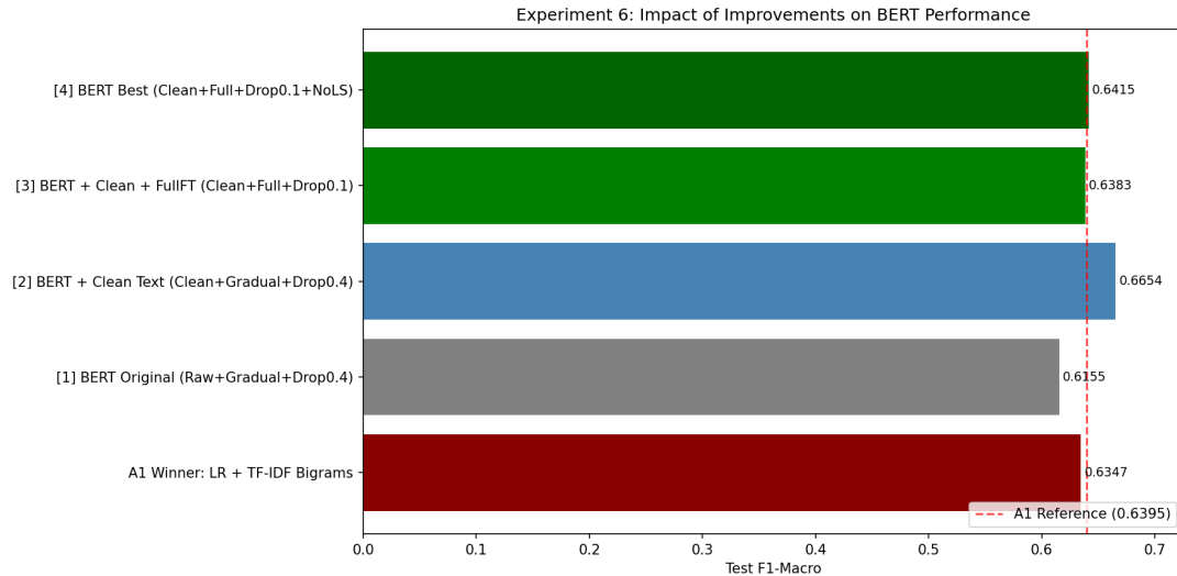
Figure 4: Visual comparison of BERT performance after improvements. Clean text is the main driver of performance.
