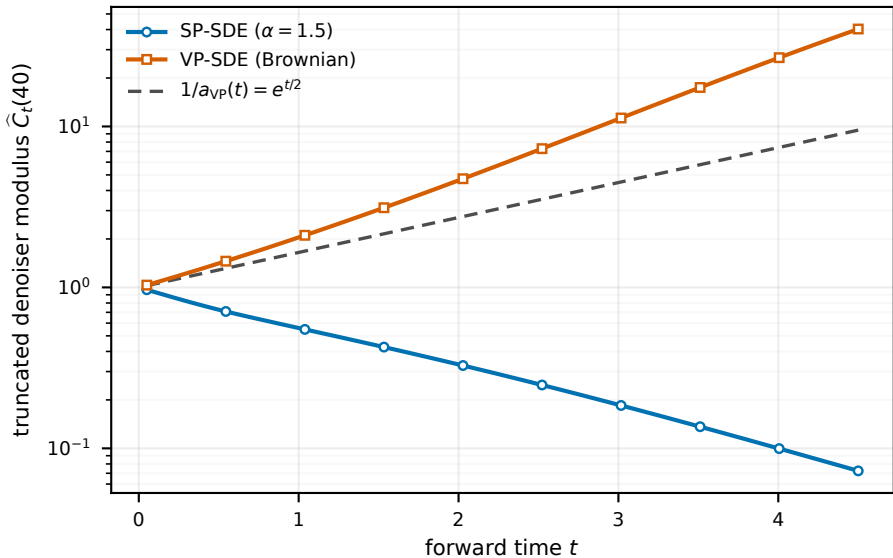
Student- t_4 target
