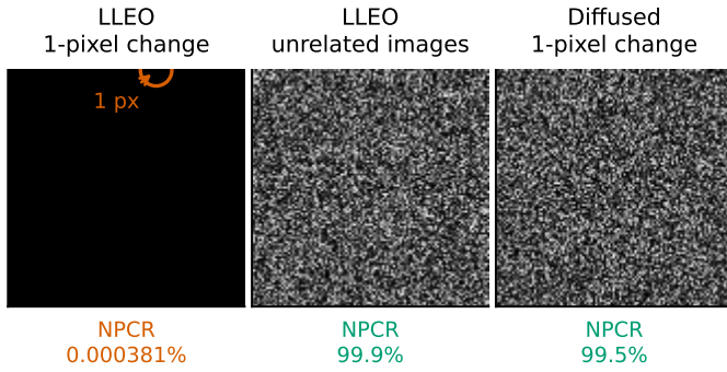
Fig. 3. Why LLEO’s reported NPCR is illusory: the absolute ciphertext difference |C_0 - C_1| (black = unchanged, bright = changed), under one fixed key. (left) A one-pixel plaintext change alters exactly one ciphertext pixel (ringed)—no diffusion—so the true one-pixel NPCR is 100/MN \approx 0.000381\% . (centre) The \approx 99.6\% LLEO reports is really the difference between two unrelated images (here 99.8833\% ), which any near-uniform cipher attains and which says nothing about plaintext sensitivity. (right) Seeding the keystream from SHA-256 of the plaintext diffuses the same one-pixel change into full noise—what a one-pixel NPCR should measure.
