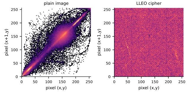
Fig. 5. Adjacent-pixel correlation as a 2D density (every horizontal pixel pair, log counts): the plain image concentrates on the diagonal—neighbours are alike—while the LLEO cipher fills the plane uniformly (Cameraman).
