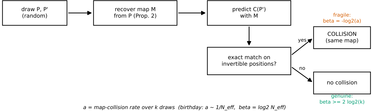
Fig. 10: The black-box \beta estimator, tied to Proposition 2. Draw two random plaintexts, recover the equivalent map from one, and test whether it predicts the other’s ciphertext exactly on the invertible positions. A match is a map-collision (same map): observed collisions give a point estimate \beta = -\log_2 a ; no collision in k draws certifies the lower bound \beta \geq 2\log_2 k . The decision rule “collision = fragile, no collision = genuine” is the whole metric.
