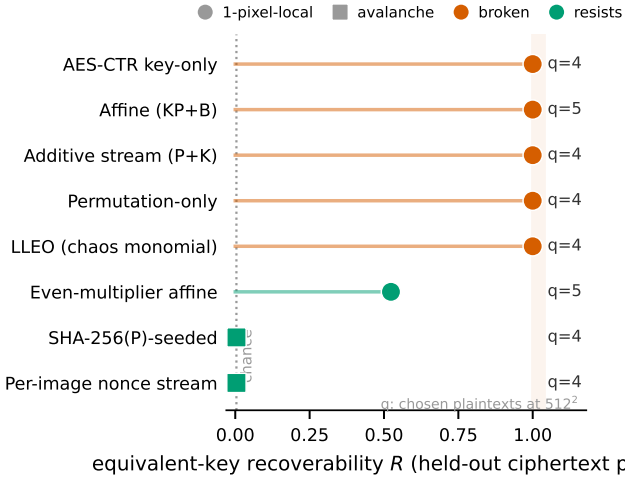
Fig. 7: Structural-audit panel: equivalent-key recoverability R per scheme (circle = one-pixel-local, square = avalanche; red = broken, green = resists), with the chosen-plaintext count at 512^2 . Every key-only scheme sits at R=1 ; only binding the keystream to the plaintext or a nonce escapes to R \approx chance.
