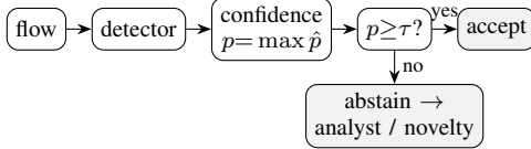
Fig. 1. The selective-prediction (reject-option) wrapper we evaluate: accept the detector’s label when its confidence p clears a threshold \tau , otherwise abstain and defer to an analyst or a benign-only novelty stage. We ask whether p is trustworthy—and what becomes of attacks that look benign.
