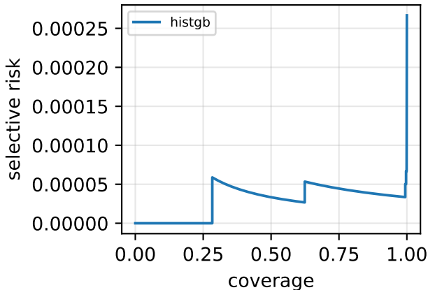
CIC-IDS-2017
