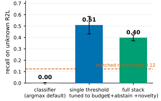
Fig. 6: The paper’s central negative result in one view. On unknown (held-out) R2L at matched analyst cost, a single budget-tuned threshold recovers 0.508 of the family, which the full abstention+novelty stack does not beat (0.397); argmax alone is blind (0.003). The operating point is the lever, not the gates. Means over K=6 seeds, 95% CIs; dashed line: the matched review load.
