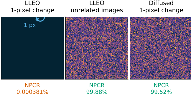
Fig. 3. The no-diffusion property, made visible (used quantitatively in Section V): the absolute ciphertext difference |C_0 - C_1| (dark = unchanged, bright = changed), under one fixed key. (left) A one-pixel plaintext change alters exactly one ciphertext pixel (ringed), no diffusion, so the true one-pixel NPCR is 100/MN \approx 0.000381\% , not the reported \approx 99.6\% . (centre) That \approx 99.6\% is really the difference between two unrelated images (here 99.88\% ), which any near-uniform cipher attains. (right) Seeding the keystream from SHA-256 of the plaintext diffuses the same one-pixel change into full noise, what a one-pixel NPCR should measure.
