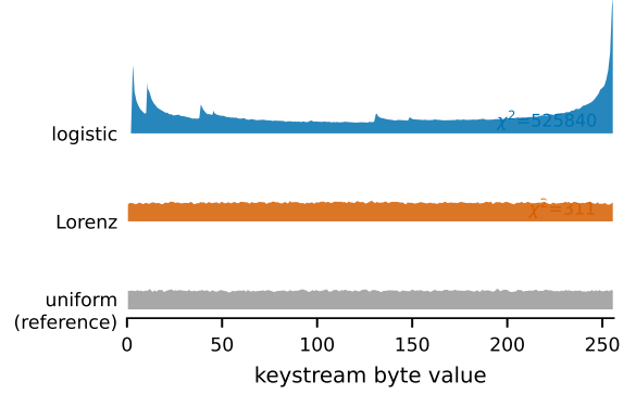
Fig. 6. Keystream byte distributions (ridgeline). The logistic keystream is sharply non-uniform (its invariant density spikes at the extremes) and even the Lorenz stream is measurably lumpy, whereas a secure stream cipher would match the flat uniform reference. A chi-square test rejects uniformity for both ( \chi^2 annotated).
