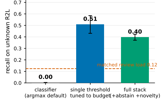
Fig. 6: The paper’s central negative result in one view. On unknown (held-out) R2L at matched analyst cost, a single budget-tuned threshold recovers 0.508 of the family—which the full abstention+novelty stack does not beat (0.397); argmax alone is blind (0.003). The operating point is the lever, not the gates. Means over K=6 seeds, 95% CIs; dashed line: the matched review load.
