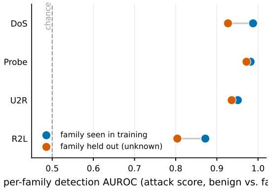
Fig. 3: Per-family detection AUROC (threshold-free), family seen vs. held out of training. Every family stays well above chance, R2L lowest but never near 0.5; the small seen \rightarrow unknown gaps are the honest size of “detection collapse” once the decision threshold is taken out of the picture.
