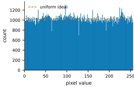
Fig. 5. Cipher histogram (Cameraman): near-uniform, yet the cipher is trivially broken.
