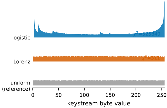
Fig. 3. Keystream byte distributions (ridgeline). The logistic keystream is sharply non-uniform—its invariant density spikes at the extremes—and even the Lorenz stream is measurably lumpy, whereas a secure stream cipher would match the flat uniform reference. A chi-square test rejects uniformity for both ( \chi^2 annotated).
