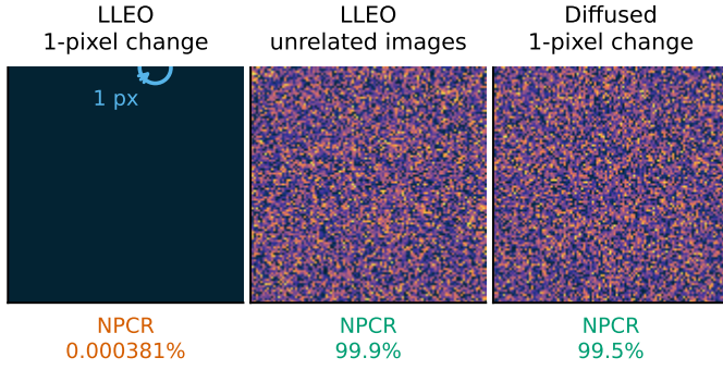
Fig. 4. Why LLEO’s reported NPCR is illusory: the absolute ciphertext difference |C_0 - C_1| (dark = unchanged, bright = changed), under one fixed key. (left) A one-pixel plaintext change alters exactly one ciphertext pixel (ringed)—no diffusion—so the true one-pixel NPCR is 100/MN \approx 0.000381\% . (centre) The \approx 99.6\% LLEO reports is really the difference between two unrelated images (here 99.8833\% ), which any near-uniform cipher attains and which says nothing about plaintext sensitivity. (right) Seeding the keystream from SHA-256 of the plaintext diffuses the same one-pixel change into full noise—what a one-pixel NPCR should measure.
