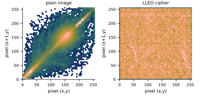
Fig. 6. Adjacent-pixel correlation as a 2D density (every horizontal pixel pair, log counts): the plain image concentrates on the diagonal—neighbours are alike—while the LLEO cipher fills the plane uniformly (Cameraman).
