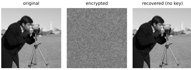
Fig. 1. Original, LLEO ciphertext, and the key-free recovery from 4 chosen plaintexts.
