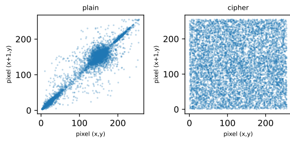
Fig. 3. Adjacent-pixel correlation, plain vs. cipher (Cameraman).
