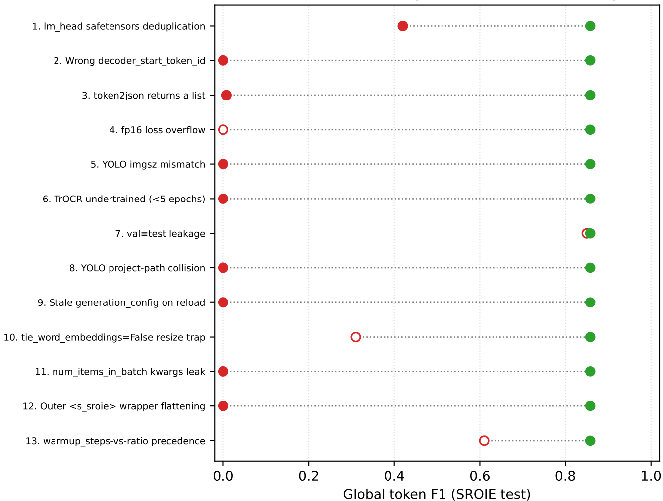
F1 before (red) vs. after (green) each of the 13 bug fixes
