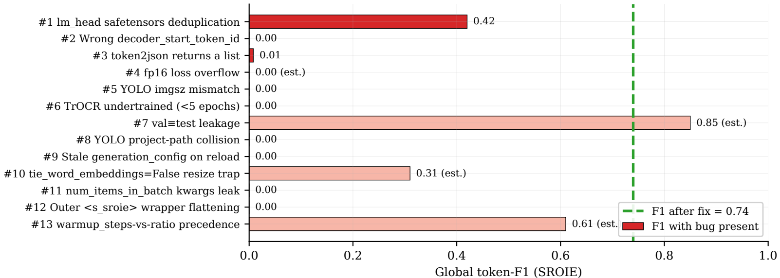
Thirteen silent F1-destroying bugs: impact before fix
