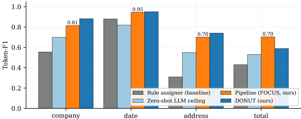
Per-field F1: rule \rightarrow LLM ceiling \rightarrow pipeline \rightarrow DONUT
