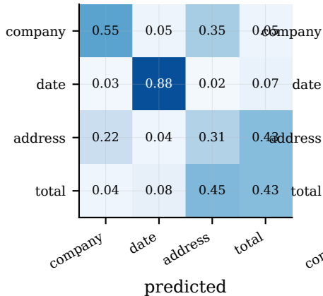
(a) Rule assigner
