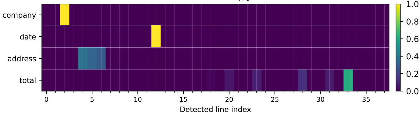
Attention-assigner cross-attention (field query → line)
