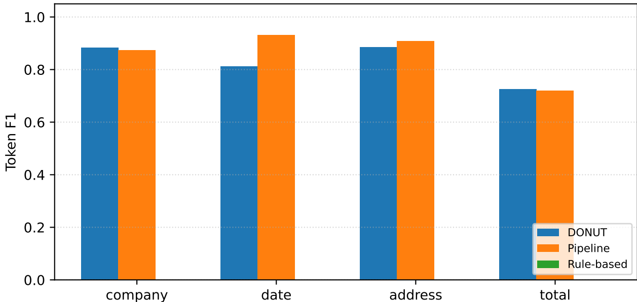
Per-field F1 by system (SROIE test split)
