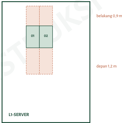
CLEARANCE RACK 1:100 (AS-ICT-06)
