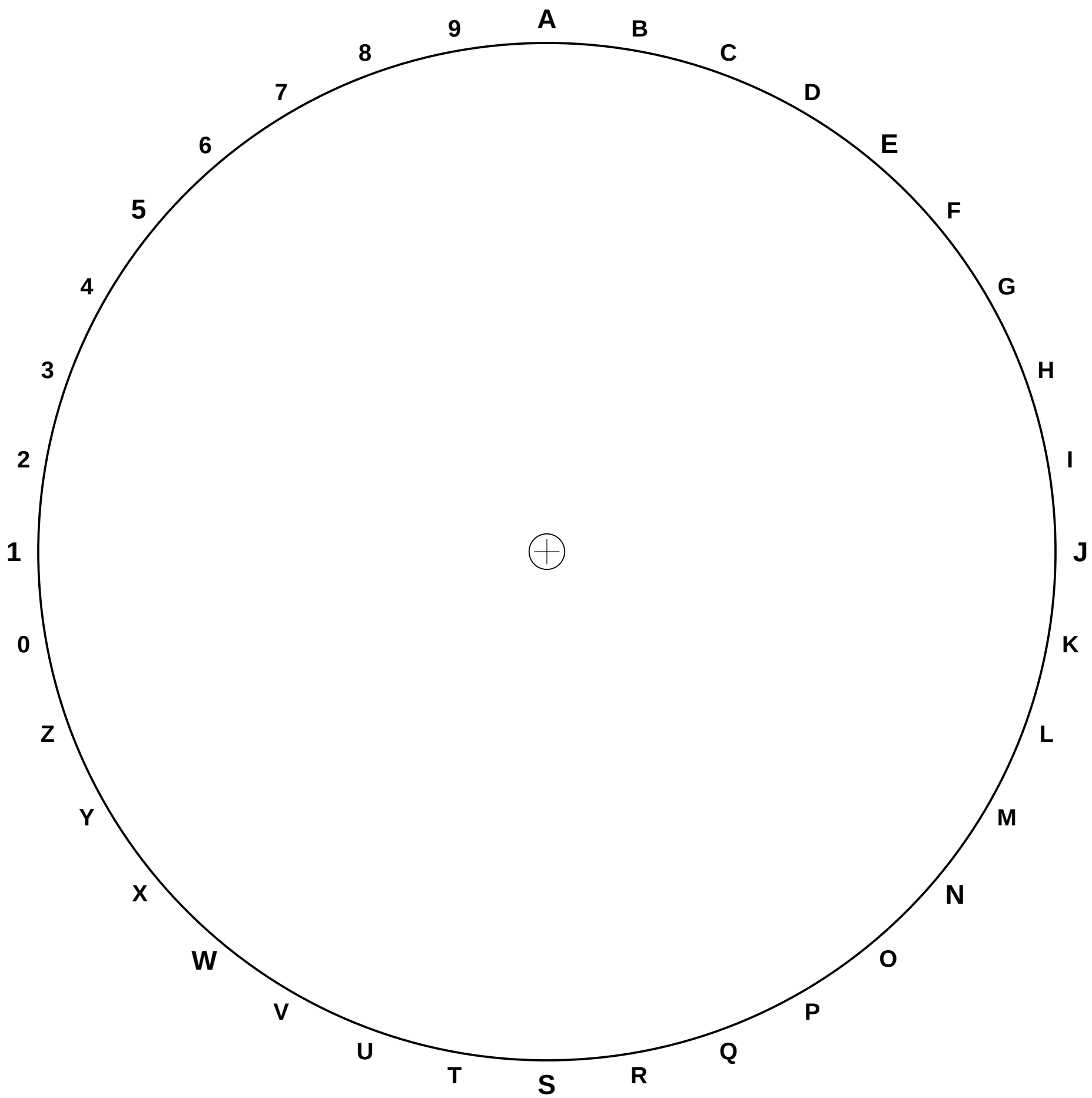
9 in dial - no spokes - 36 marks x 10 deg - A at North - print at 100% (no fit-to-page) Cut on the circle. Letters sit outside. Align the 8 mm center with the bearing.
