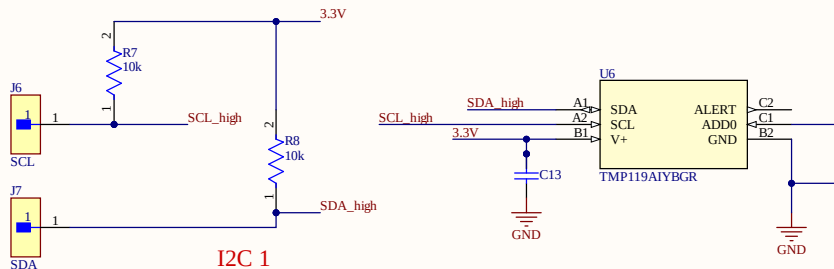
Temperature Sensor
