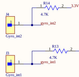
Gyro Interrupts
