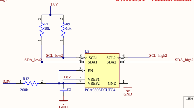
Bidirectional I2C Bus 2
