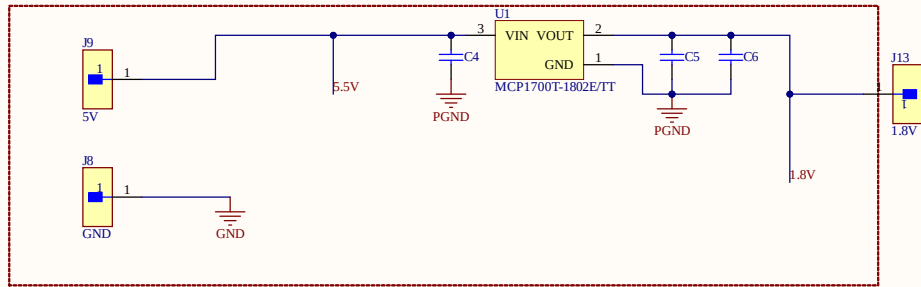
Power Stage
