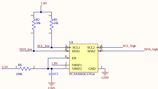
Bidirectional I2C Bus 1
