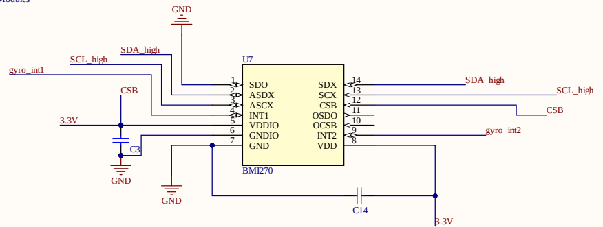
Gyroscope + Accelerometer
