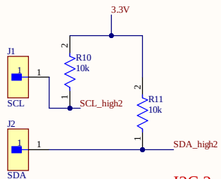
I2C 2
