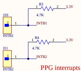
PPG interrupts
