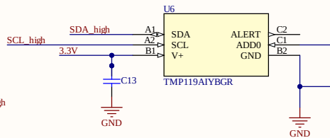
Temperature Sensor
