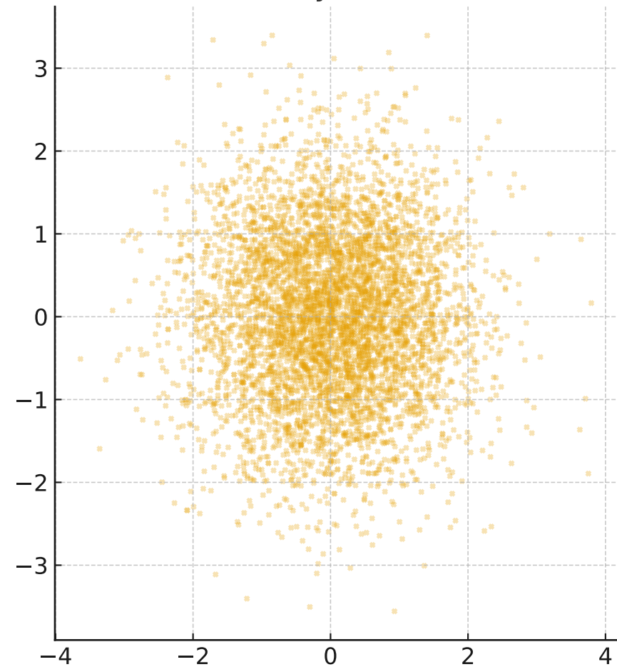
SO(3,1) Initial System Events (t-x)
