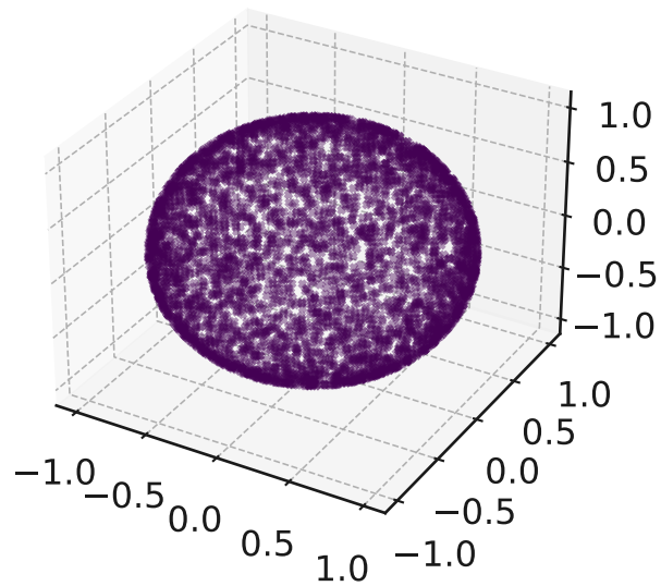
SU(2) Collapse t=10/20
