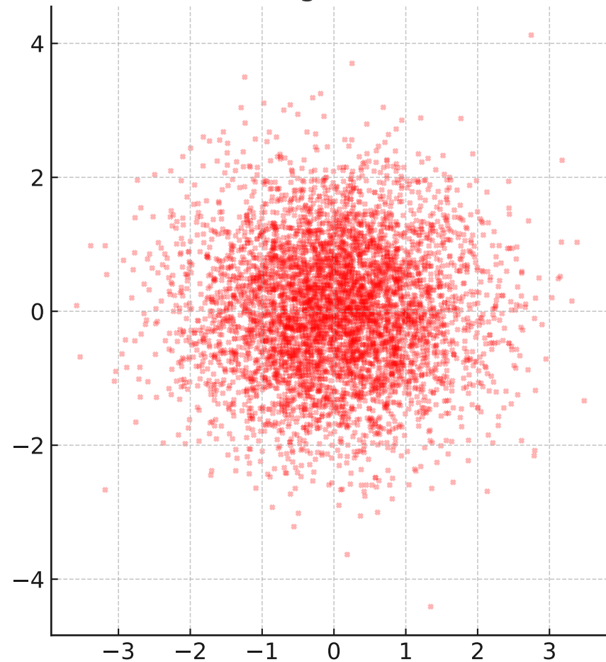
SO(3,1) Origin Events (t-x)
