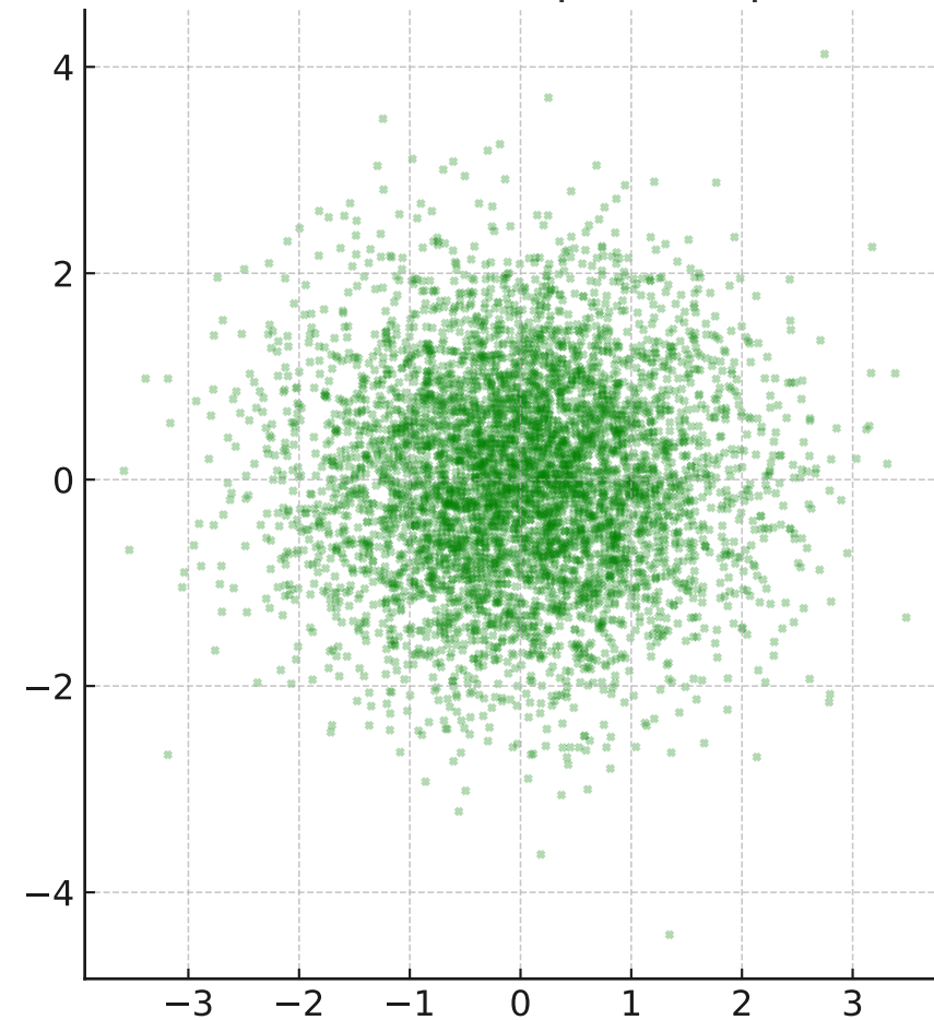
SO(3,1) Post-Collapse (t-x plane)
