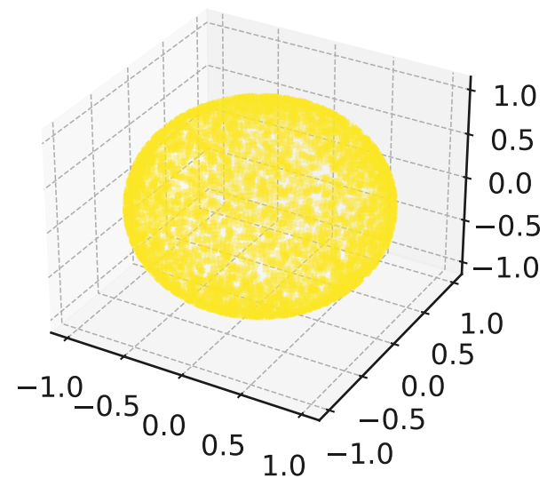
SU(2) Collapse t=20/20
