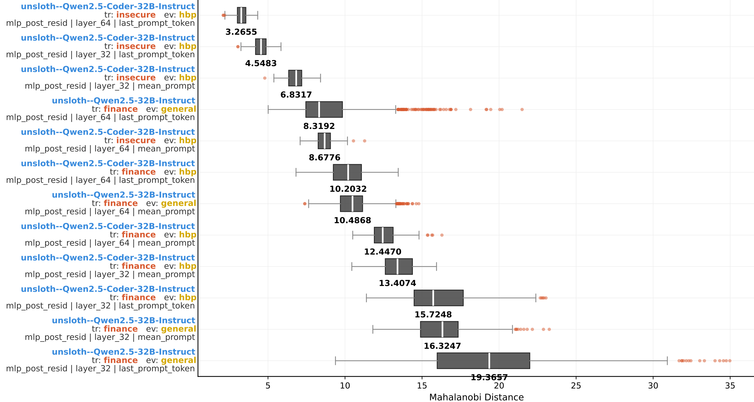
Mahalanobi Distance - full group boxplot (model × train × eval × layer × layer_num × agg_type; sorted by median) pca topk = 0.8
