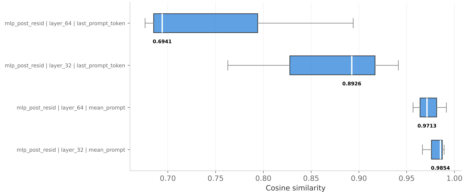
PCA reconstruction cosine - by layer & agg type — boxplot (sorted by median; label: layer | layer_num | agg_type) pca topk = 0.9
