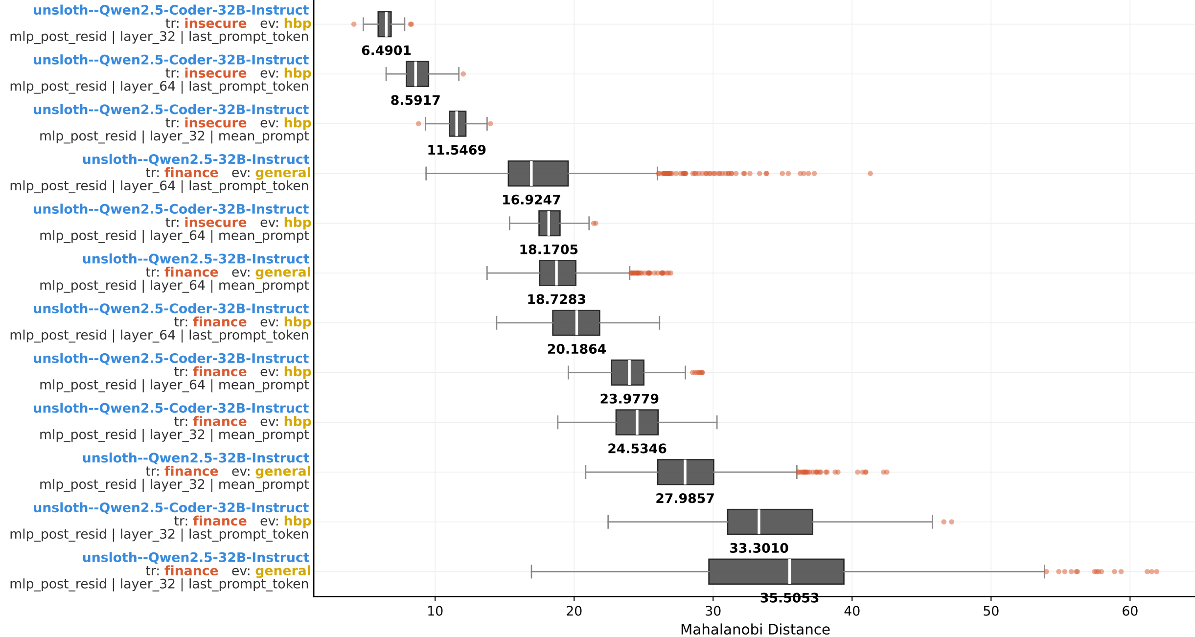
Mahalanobi Distance - full group boxplot (model × train × eval × layer × layer_num × agg_type; sorted by median) pca topk = 0.9
