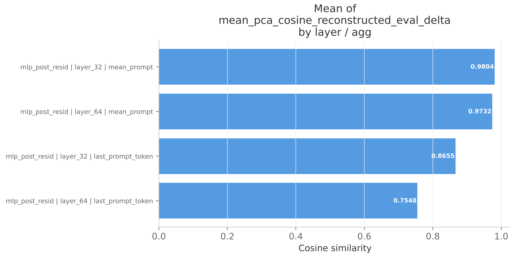
PCA reconstruction cosine by layer & agg type
