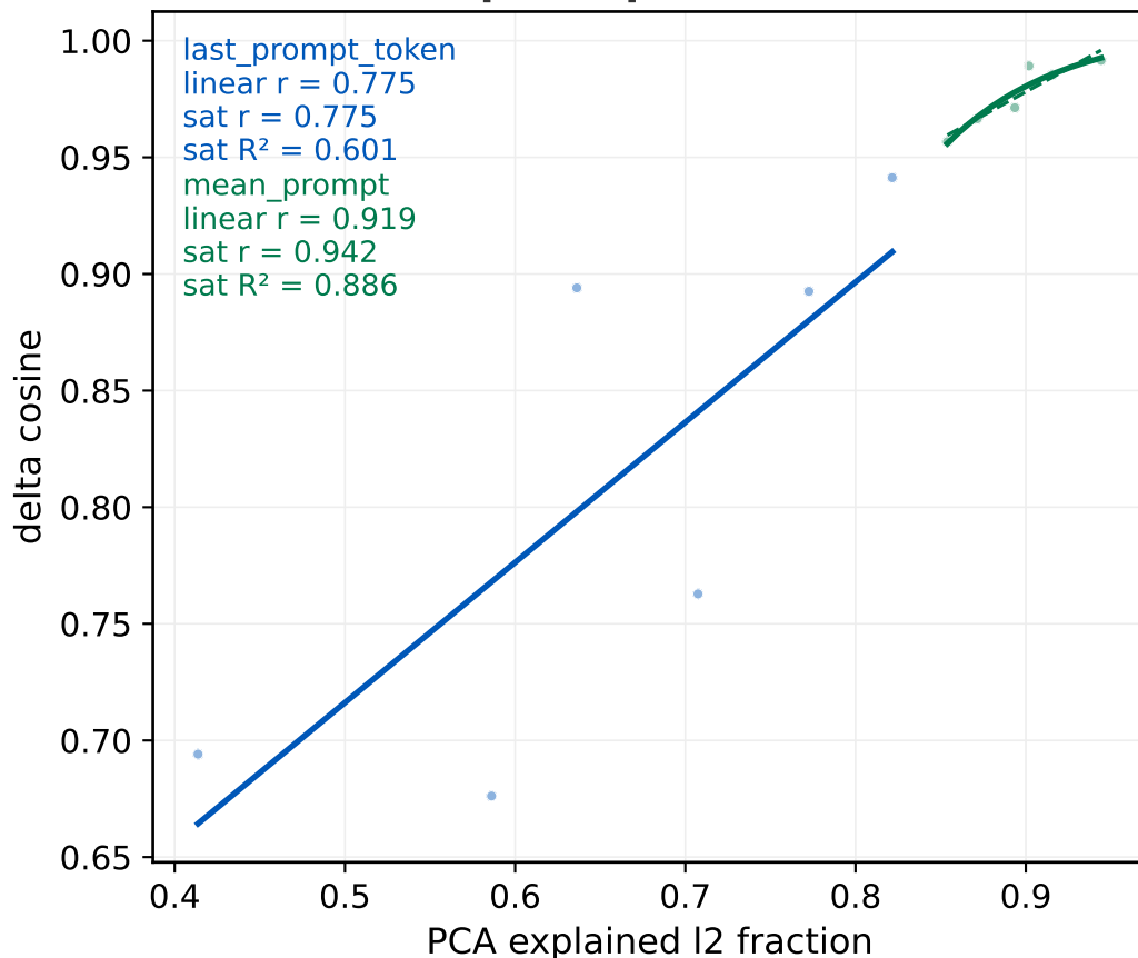
PCA explained I2 fraction vs PCA reconstruction cosine pca topk = 0.9
