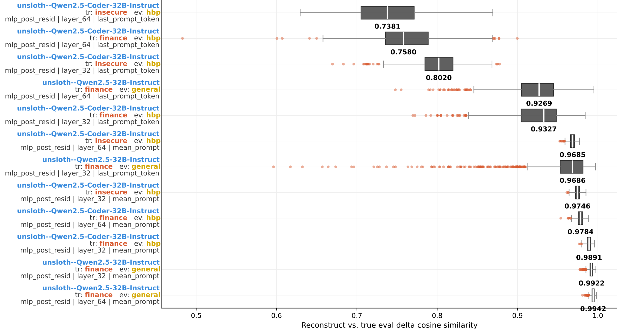
PCA reconstruction cosine - full group boxplot (model × train × eval × layer × layer_num × agg_type; sorted by median) pca topk = 0.95
