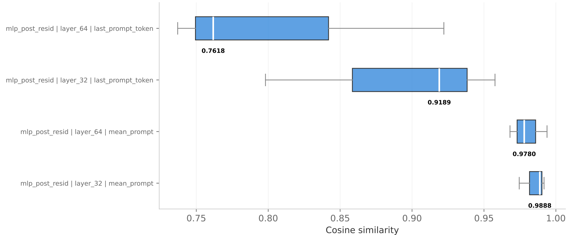
PCA reconstruction cosine - by layer & agg type — boxplot (sorted by median; label: layer | layer_num | agg_type) pca topk = 0.95
