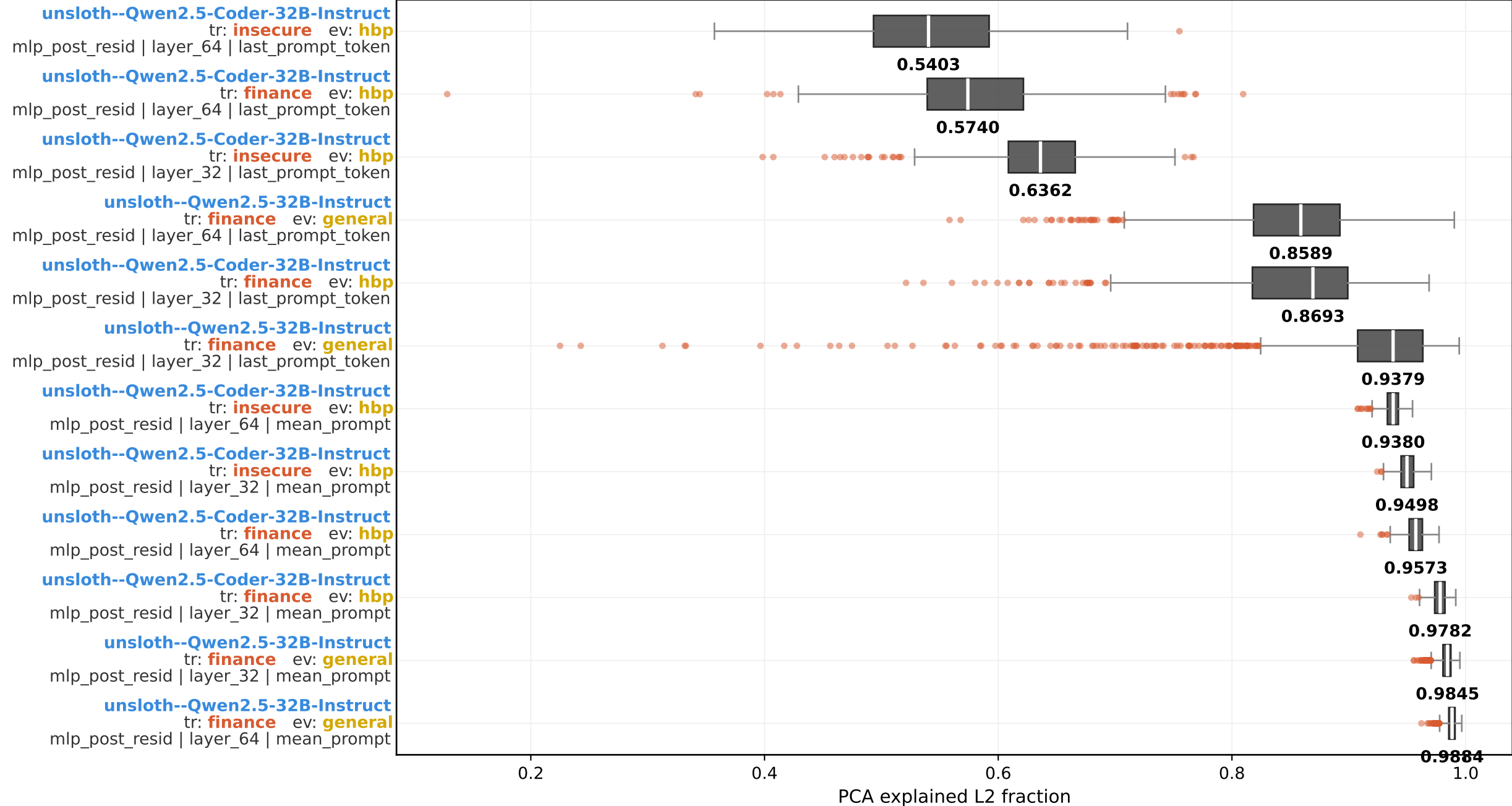
PCA explained L2 fraction - full group boxplot (model × train × eval × layer × layer_num × agg_type; sorted by median) pca topk = 0.95
