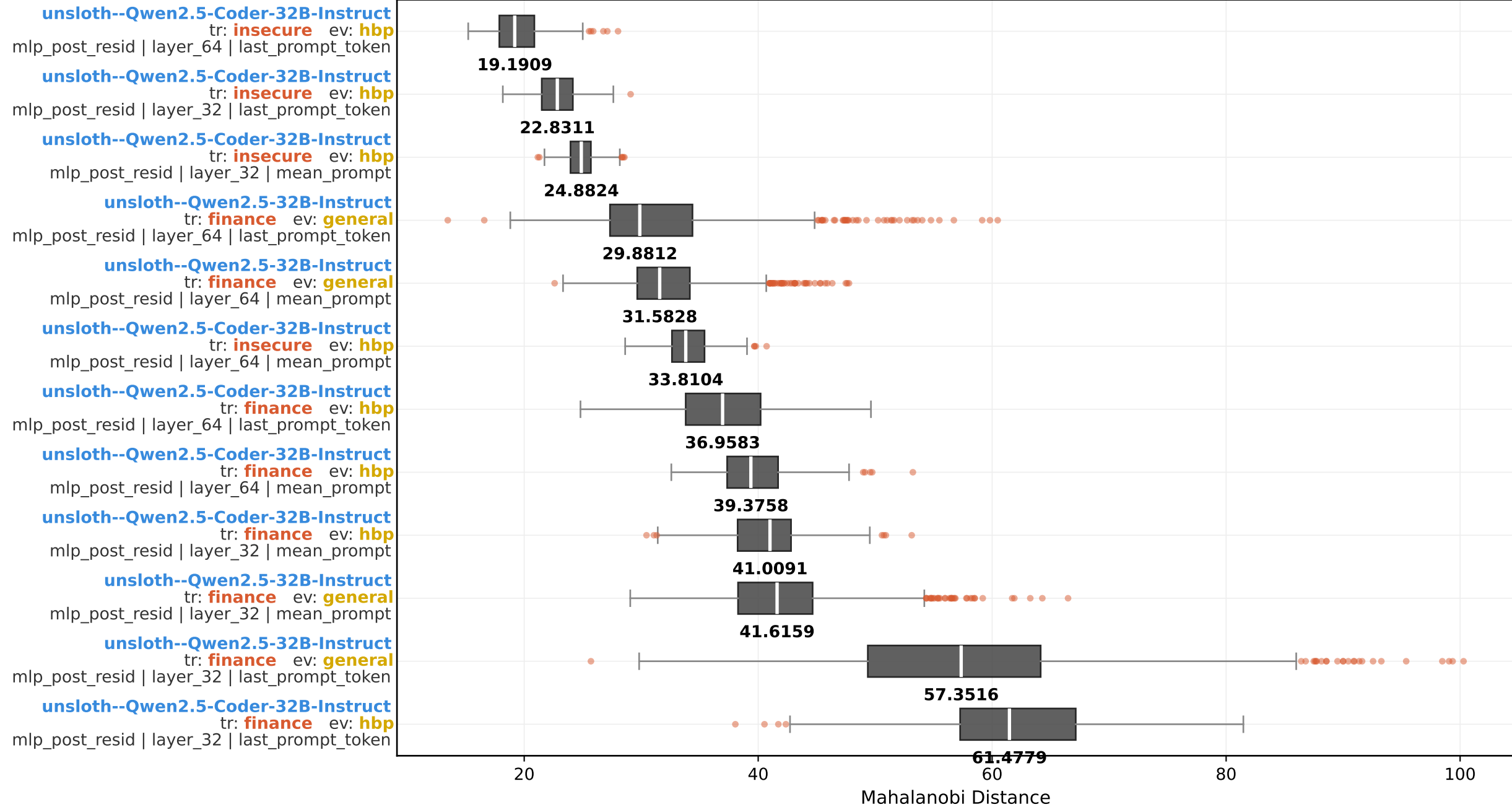
Mahalanobi Distance - full group boxplot (model × train × eval × layer × layer_num × agg_type; sorted by median) pca topk = 0.95
