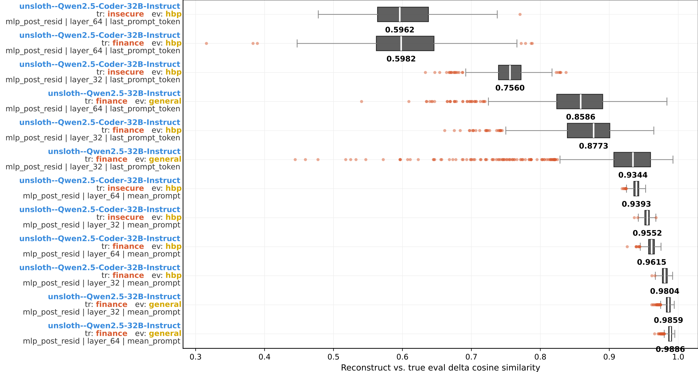
PCA reconstruction cosine - full group boxplot (model × train × eval × layer × layer_num × agg_type; sorted by median) pca topk = 0.8
