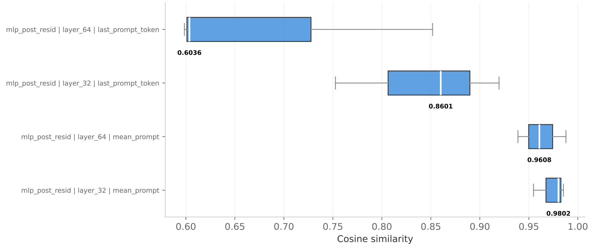
PCA reconstruction cosine - by layer & agg type — boxplot (sorted by median; label: layer | layer_num | agg_type) pca topk = 0.8
