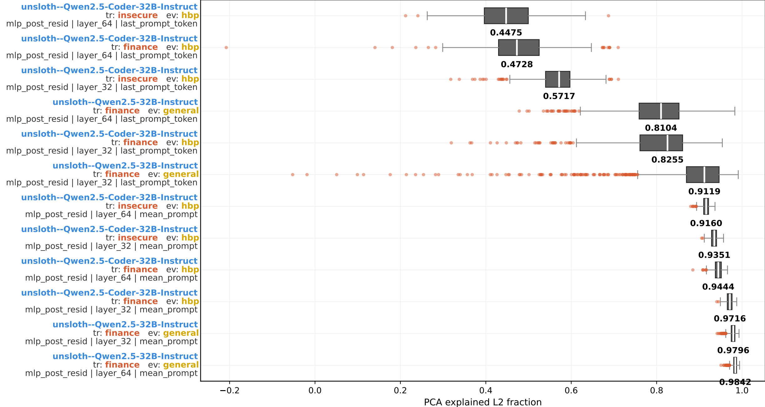
PCA explained L2 fraction - full group boxplot (model × train × eval × layer × layer_num × agg_type; sorted by median) pca topk = 0.9
