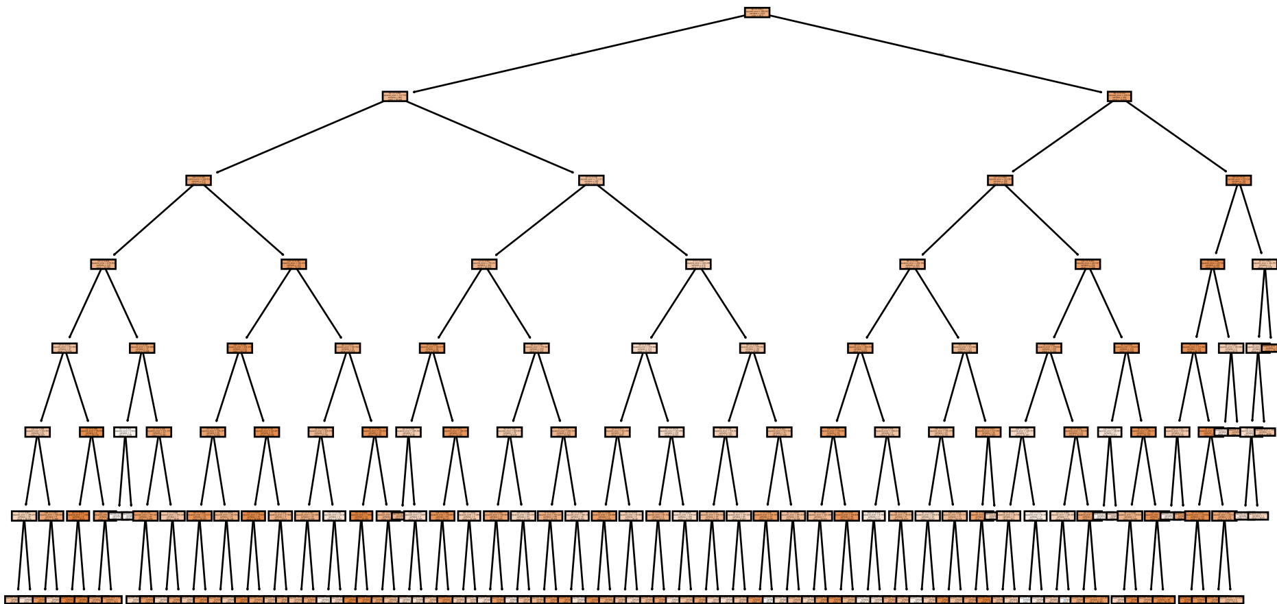
Decision Tree (target=harmless, feature=pretrained.random_projections.1.eval_var, R^2=0.6862 )
