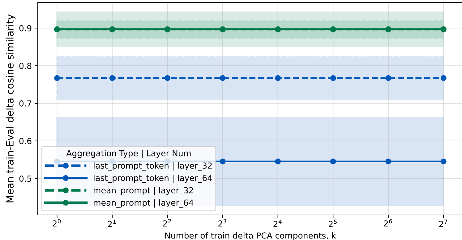
Mean train-Eval delta cosine similarity across k by Aggregation Type and Layer Num averaged over three model|train data|eval data combinations
