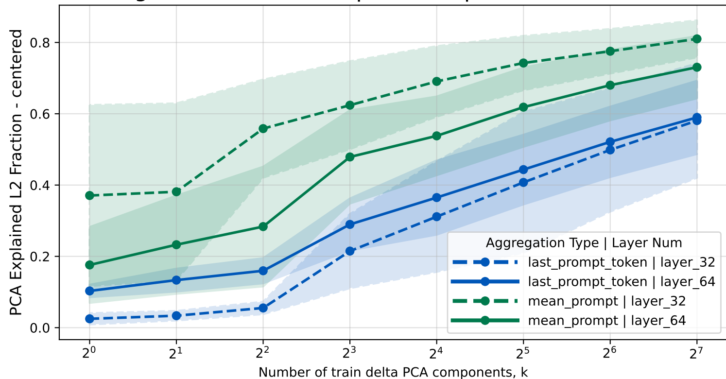
PCA Explained L2 Fraction - centered across k by Aggregation Type and Layer Num averaged over three model|train data|eval data combinations
